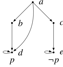
Figure 1: Model for example formula with global modalities.
