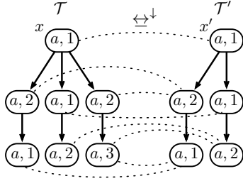
Figure 7: key(a) not in XPath_{=}^{\uparrow\downarrow*} .
