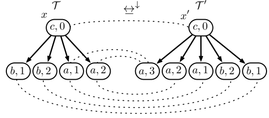
Figure 8: fk(a,b) not in XPath_{=}^{\downarrow\downarrow*} .
