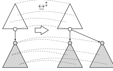
Figure 6: Closure under subtree replication.
