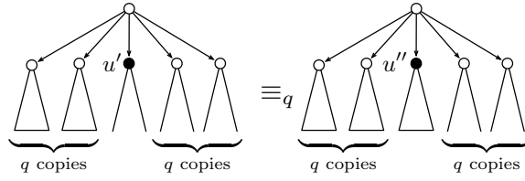
Figure 4: Definition of \mathcal{T}' , u' and \mathcal{T}'' , u'' .
