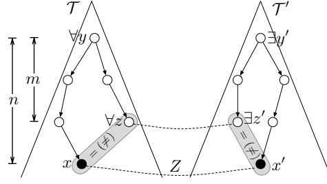
Figure 3: Zig clause of bisimulation for \text{XPath}_{\equiv}^{\downarrow}
