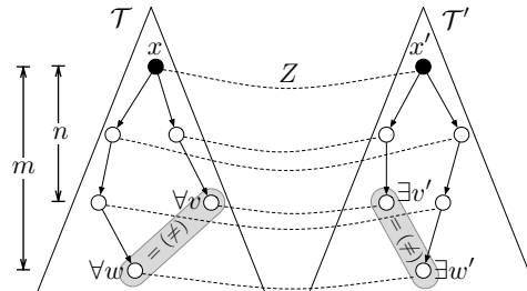
Figure 2: Zig clause of bisimulation for XPath_{\downarrow}^{\downarrow} .
