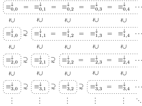
Figure 5: Hierarchy of \text{XPath}_{\downarrow} .
