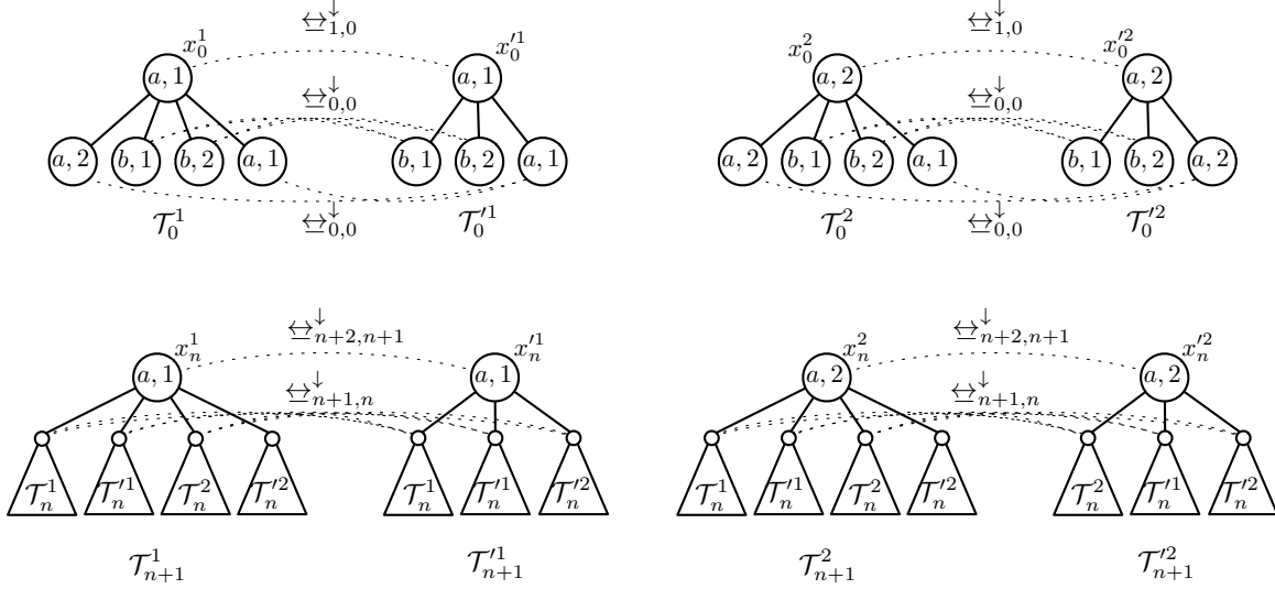
Figure 12: Definition of data trees \mathcal{T}_n^i , \mathcal{T}_n^{i'} ( n \geq 0, i \in \{1, 2\} ) for proof of Theorem 7.
