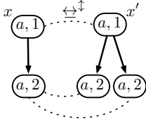
Figure 7: key(a) not in XPath_{=}^{\uparrow\downarrow*} .
