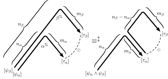
Figure 10: Normal form for data tests.
