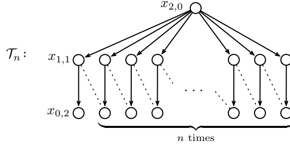
Figure 11: Model verifying \psi_i^j for all i \geq n and not verifying \varphi_l for no l < n . Dotted lines represent equal data values.
